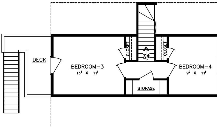
SECOND FLOOR
